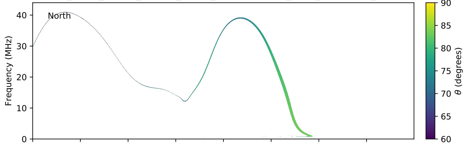
expres_earth_jupiter_europa_jrm09_lossc-wid1deg_3kev_20071105_v01.cdf
