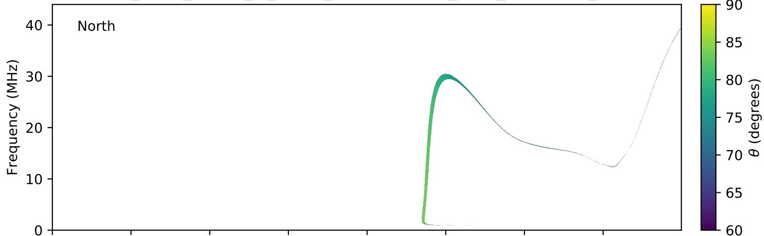
expres_earth_jupiter_io_jrm09_lossc-wid1deg_3kev_20071028_v01.cdf
