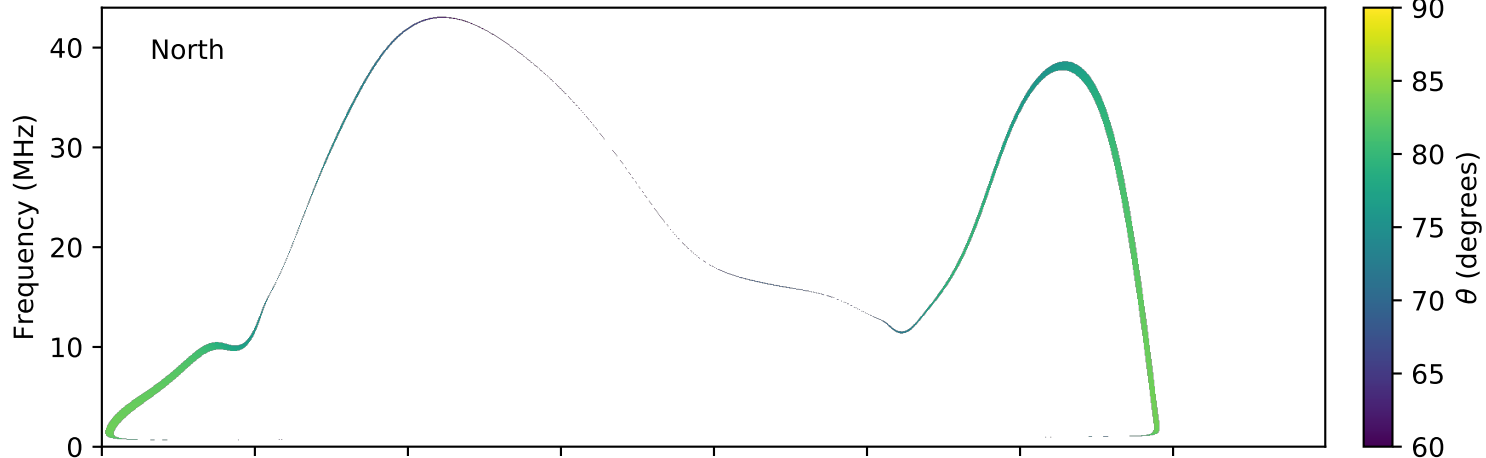
expres_earth_jupiter_io_jrm09_lossc-wid1deg_3kev_20071025_v01.cdf
