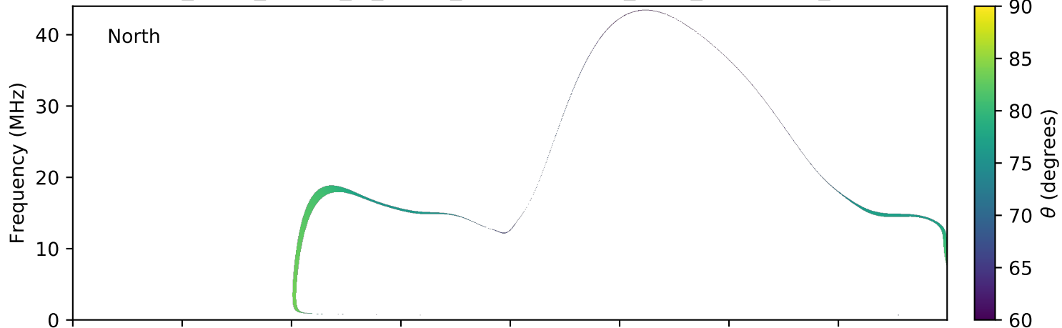
expres_earth_jupiter_io_jrm09_lossc-wid1deg_3kev_20071023_v01.cdf
