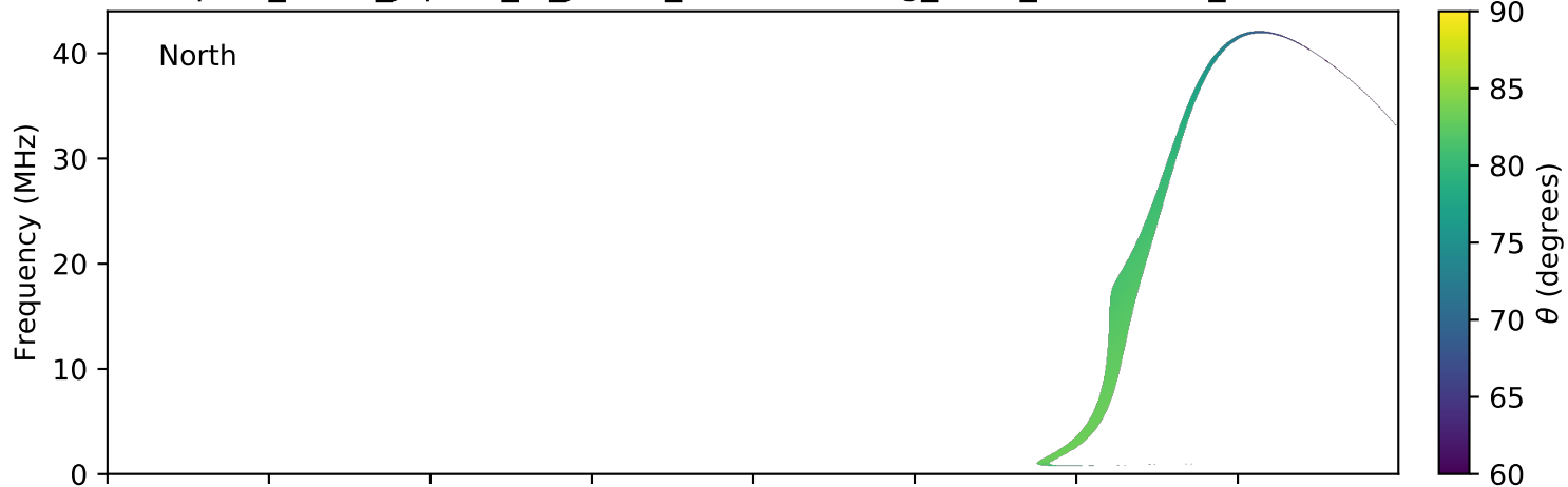
expres_earth_jupiter_io_jrm09_lossc-wid1deg_3kev_20071019_v01.cdf
