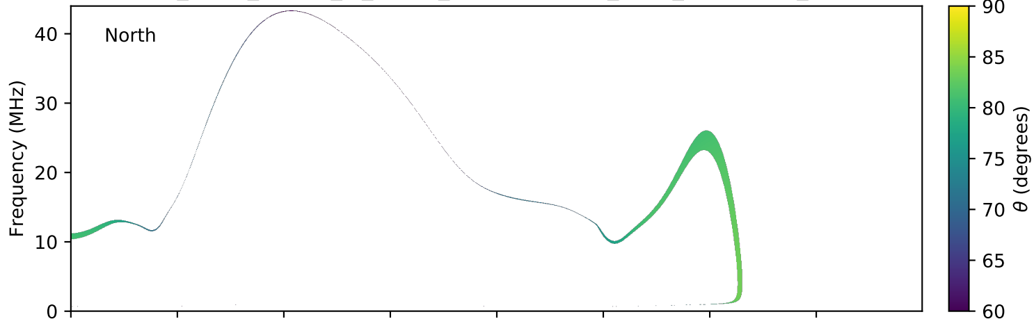
expres_earth_jupiter_io_jrm09_lossc-wid1deg_3kev_20071018_v01.cdf
