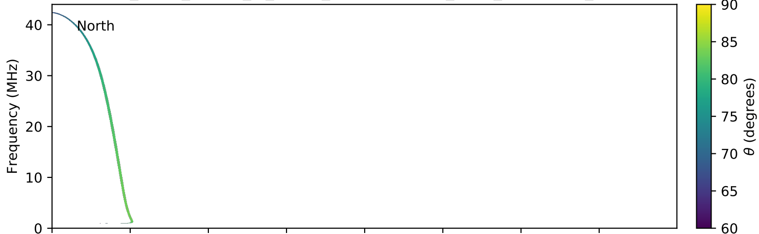
expres_earth_jupiter_io_jrm09_lossc-wid1deg_3kev_20071008_v01.cdf
