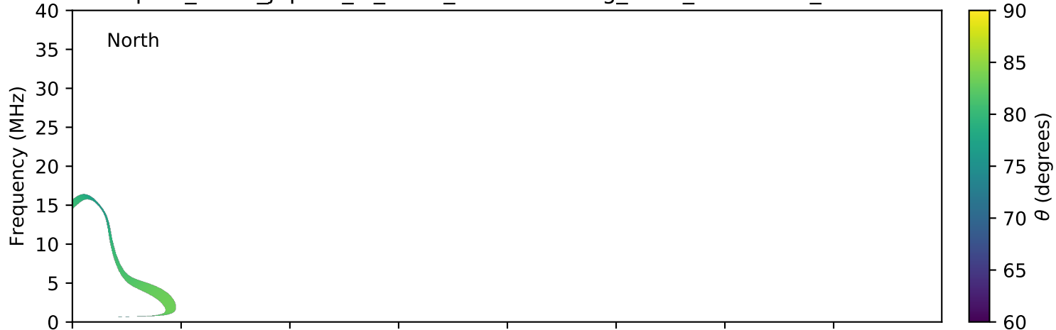
expres_earth_jupiter_io_isaac_lossc-wid1deg_3kev_20071031_v01.cdf
