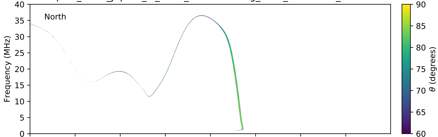
expres_earth_jupiter_io_isaac_lossc-wid1deg_3kev_20071027_v01.cdf
