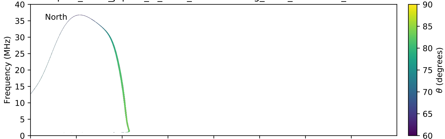
expres_earth_jupiter_io_isaac_lossc-wid1deg_3kev_20071022_v01.cdf
