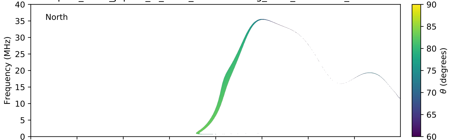
expres_earth_jupiter_io_isaac_lossc-wid1deg_3kev_20071021_v01.cdf
