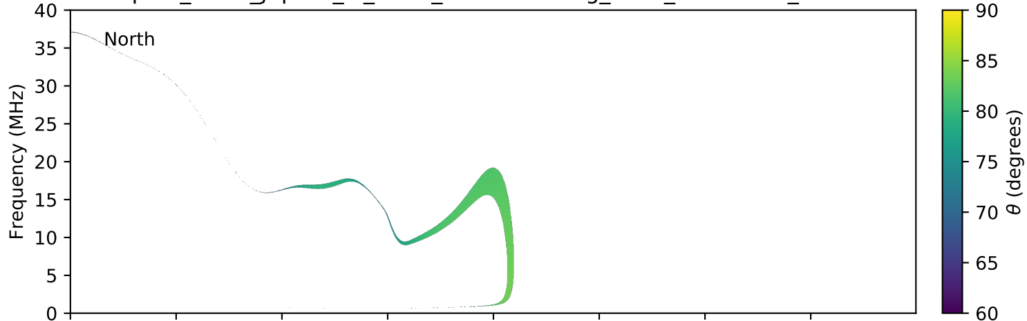
expres_earth_jupiter_io_isaac_lossc-wid1deg_3kev_20071020_v01.cdf
