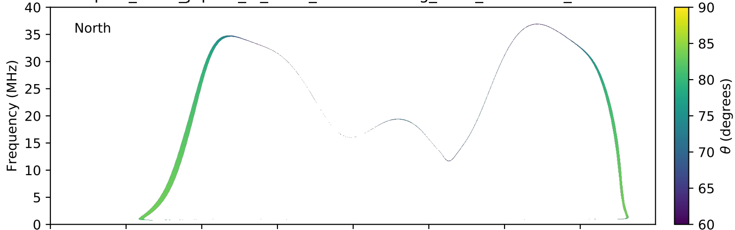
expres_earth_jupiter_io_isaac_lossc-wid1deg_3kev_20071016_v01.cdf
