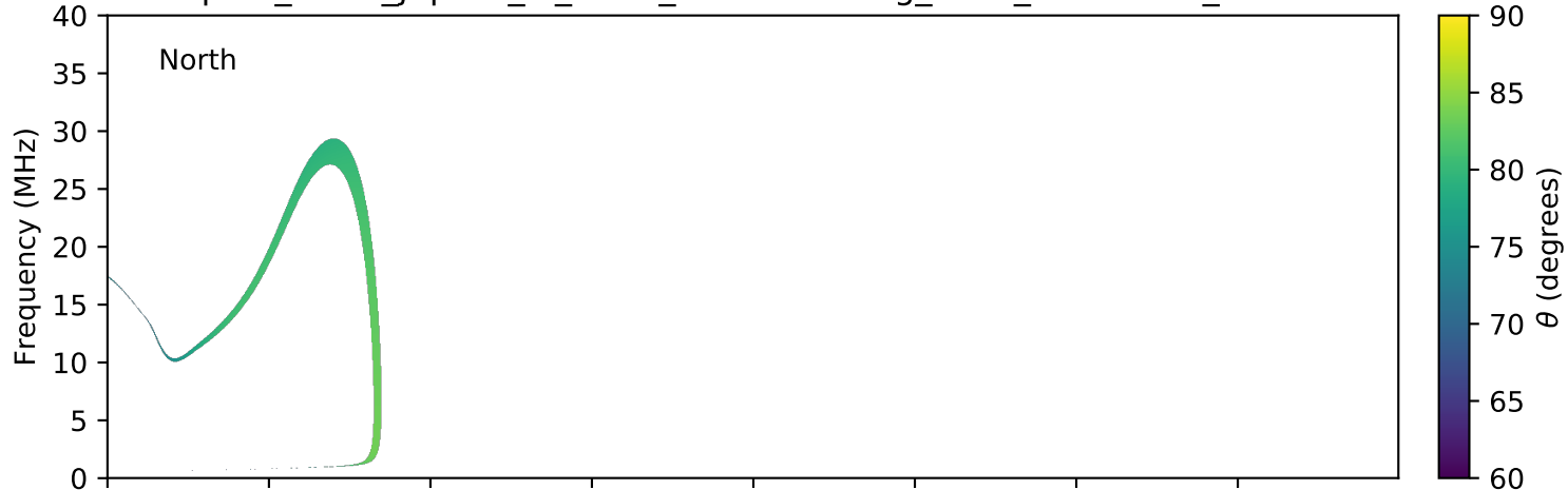
expres_earth_jupiter_io_isaac_lossc-wid1deg_3kev_20071015_v01.cdf
