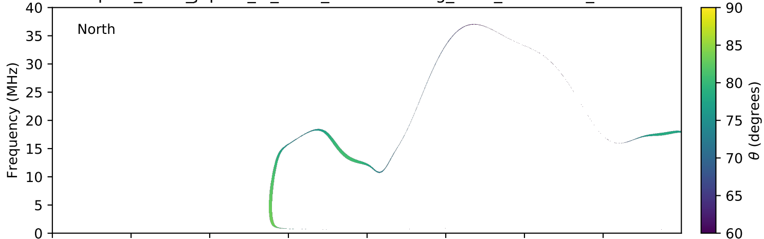
expres_earth_jupiter_io_isaac_lossc-wid1deg_3kev_20071014_v01.cdf
