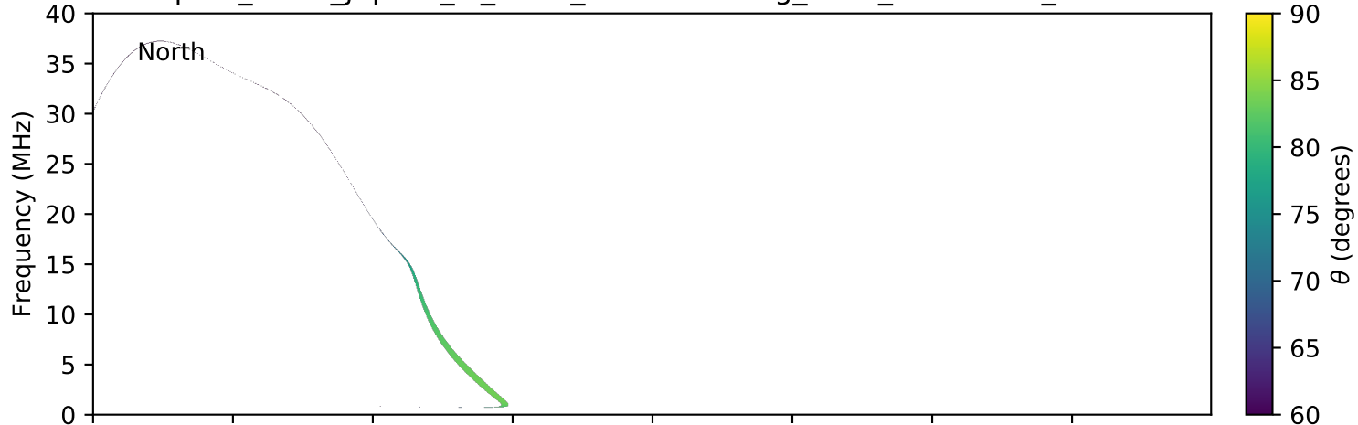
expres_earth_jupiter_io_isaac_lossc-wid1deg_3kev_20071013_v01.cdf
