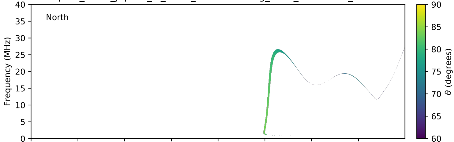
expres_earth_jupiter_io_isaac_lossc-wid1deg_3kev_20071012_v01.cdf
