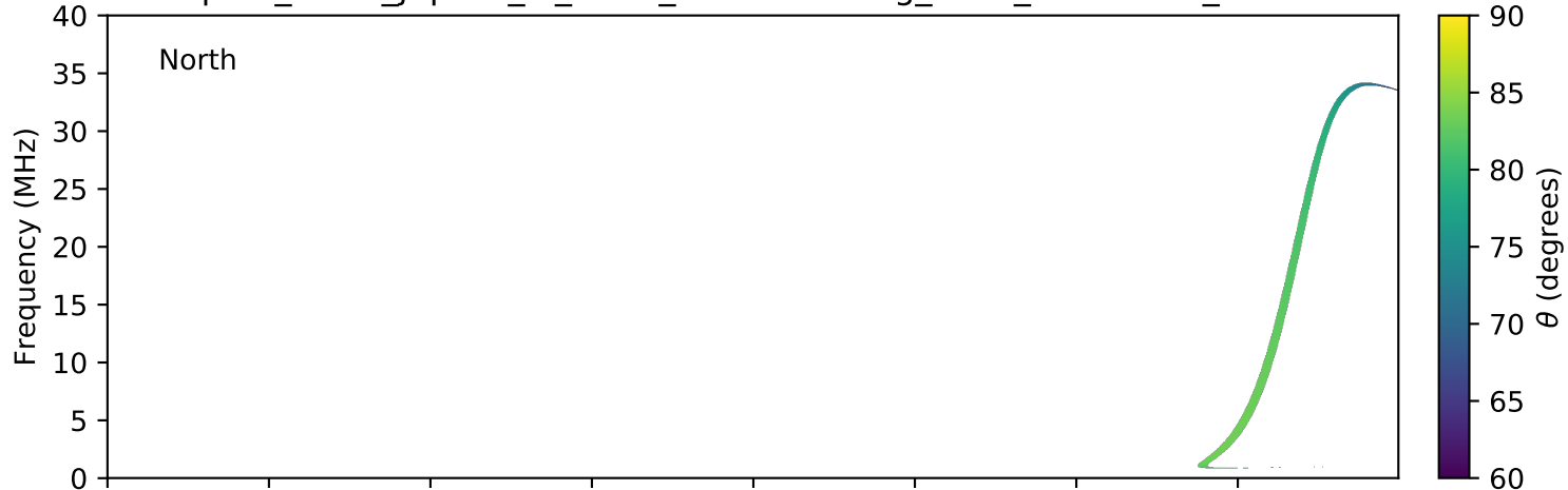
expres_earth_jupiter_io_isaac_lossc-wid1deg_3kev_20071010_v01.cdf
