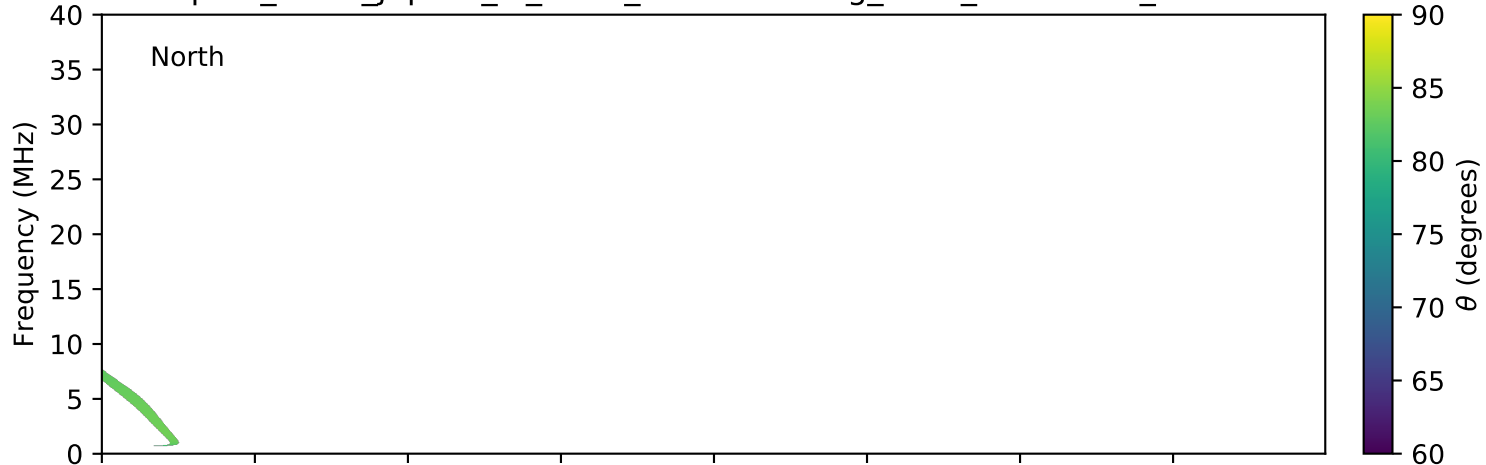
expres_earth_jupiter_io_isaac_lossc-wid1deg_3kev_20071008_v01.cdf
