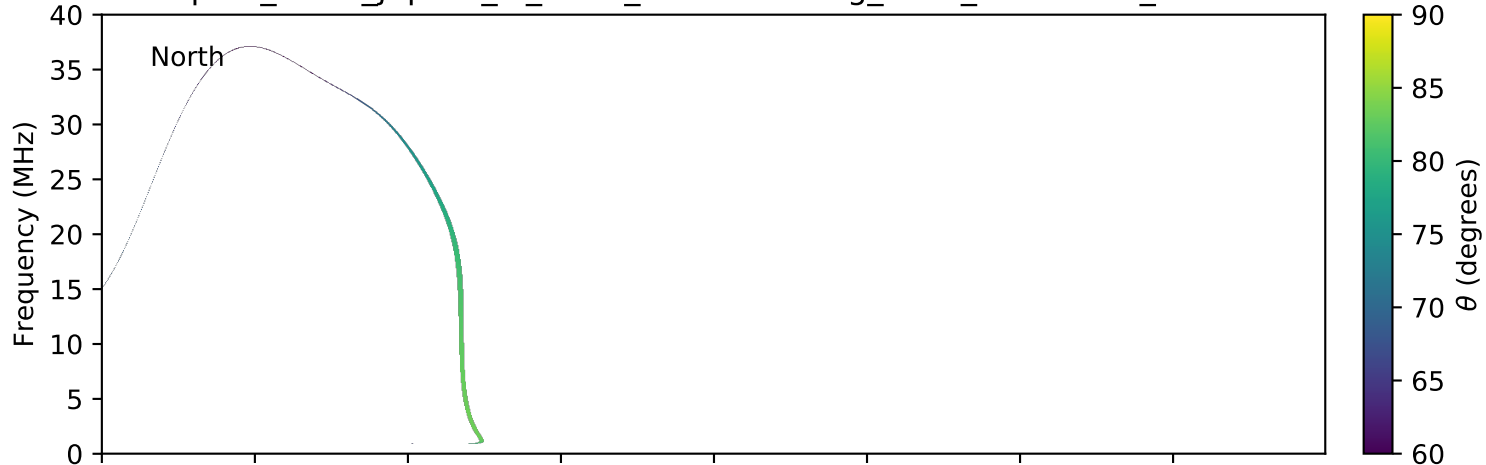
expres_earth_jupiter_io_isaac_lossc-wid1deg_3kev_20071006_v01.cdf
