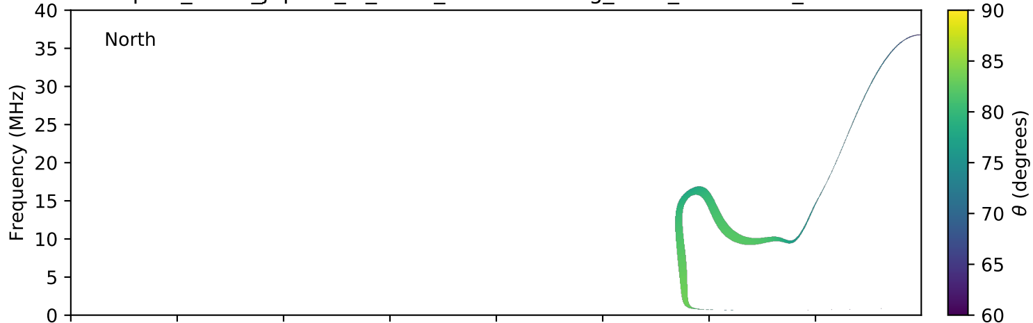
expres_earth_jupiter_io_isaac_lossc-wid1deg_3kev_20071003_v01.cdf
