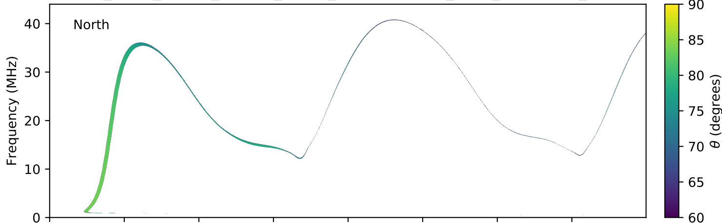
expres_earth_jupiter_europa_jrm09_lossc-wid1deg_3kev_20071021_v01.cdf
