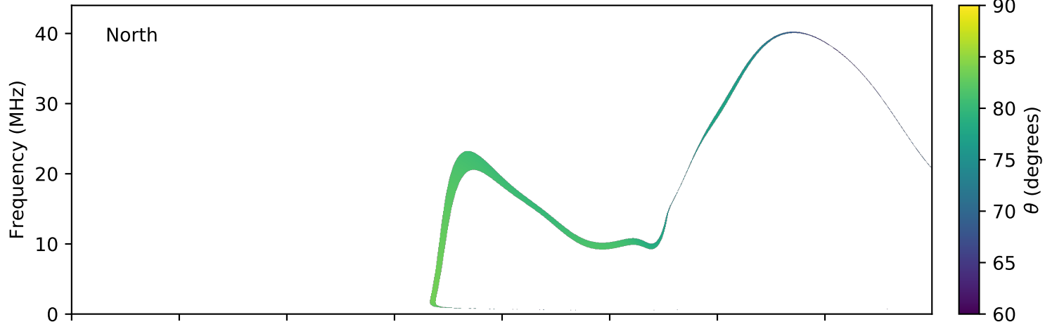
expres_earth_jupiter_europa_jrm09_lossc-wid1deg_3kev_20071017_v01.cdf
