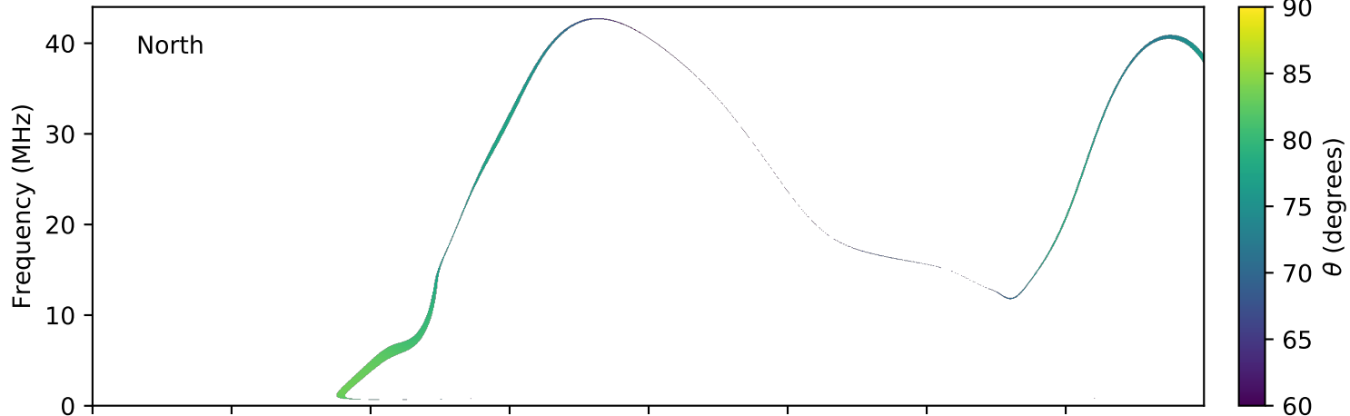
expres_earth_jupiter_io_jrm09_lossc-wid1deg_3kev_20070930_v01.cdf
