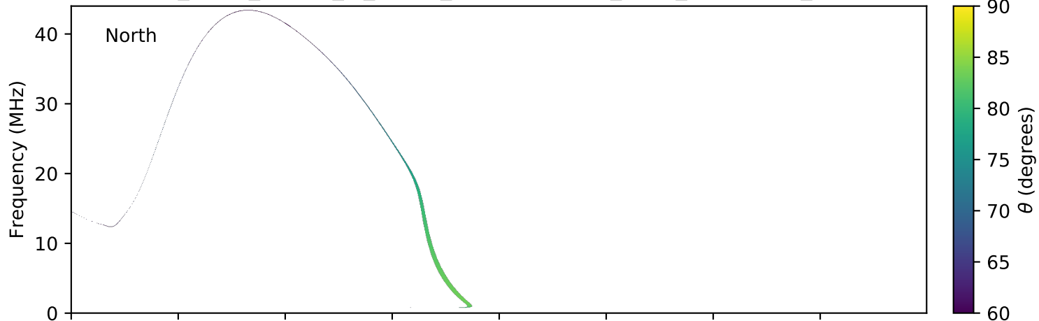
expres_earth_jupiter_io_jrm09_lossc-wid1deg_3kev_20070927_v01.cdf
