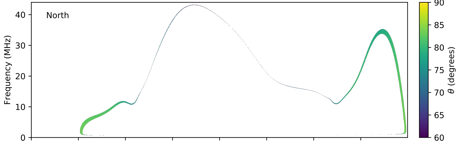
expres_earth_jupiter_io_jrm09_lossc-wid1deg_3kev_20070923_v01.cdf
