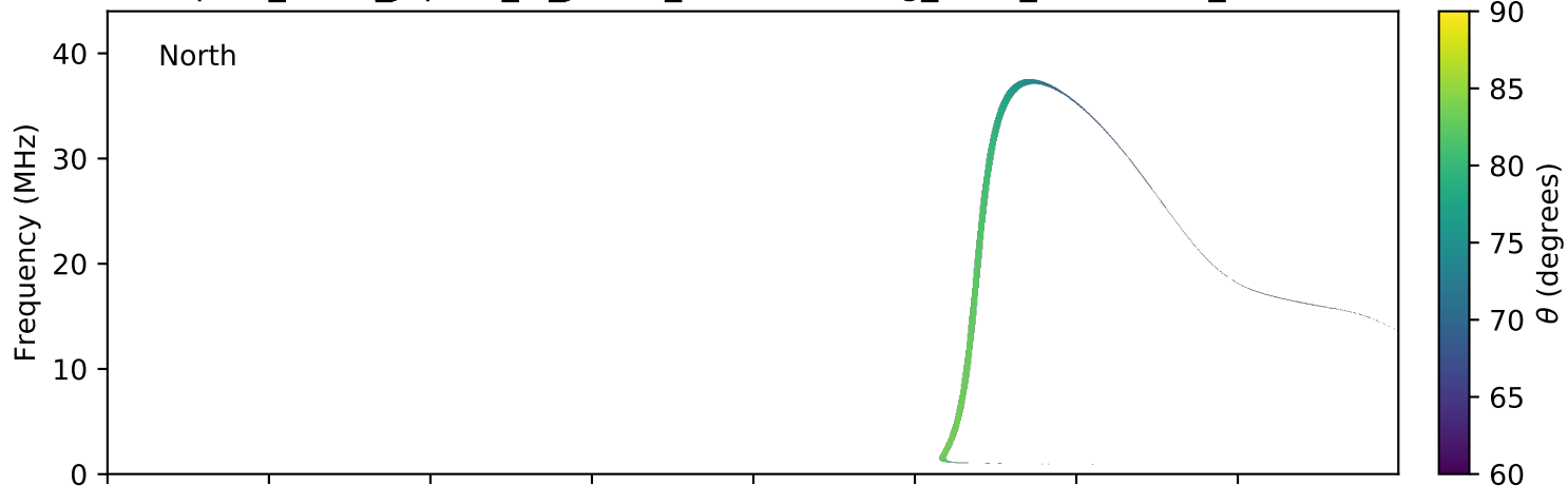
expres_earth_jupiter_io_jrm09_lossc-wid1deg_3kev_20070919_v01.cdf
