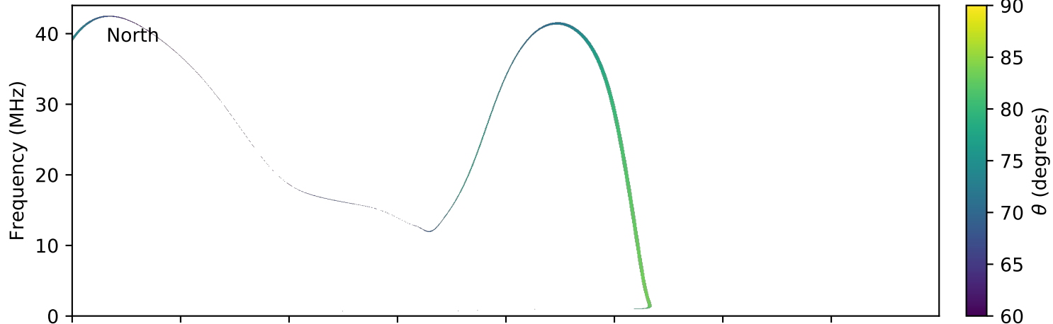
expres_earth_jupiter_io_jrm09_lossc-wid1deg_3kev_20070918_v01.cdf
