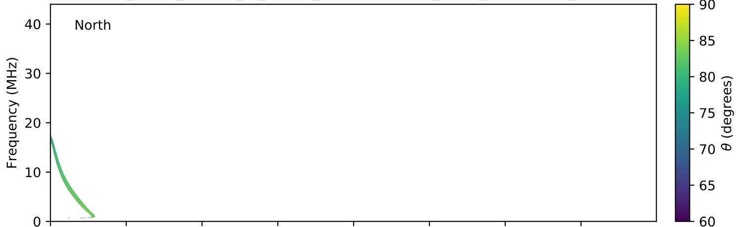
expres_earth_jupiter_io_jrm09_lossc-wid1deg_3kev_20070915_v01.cdf
