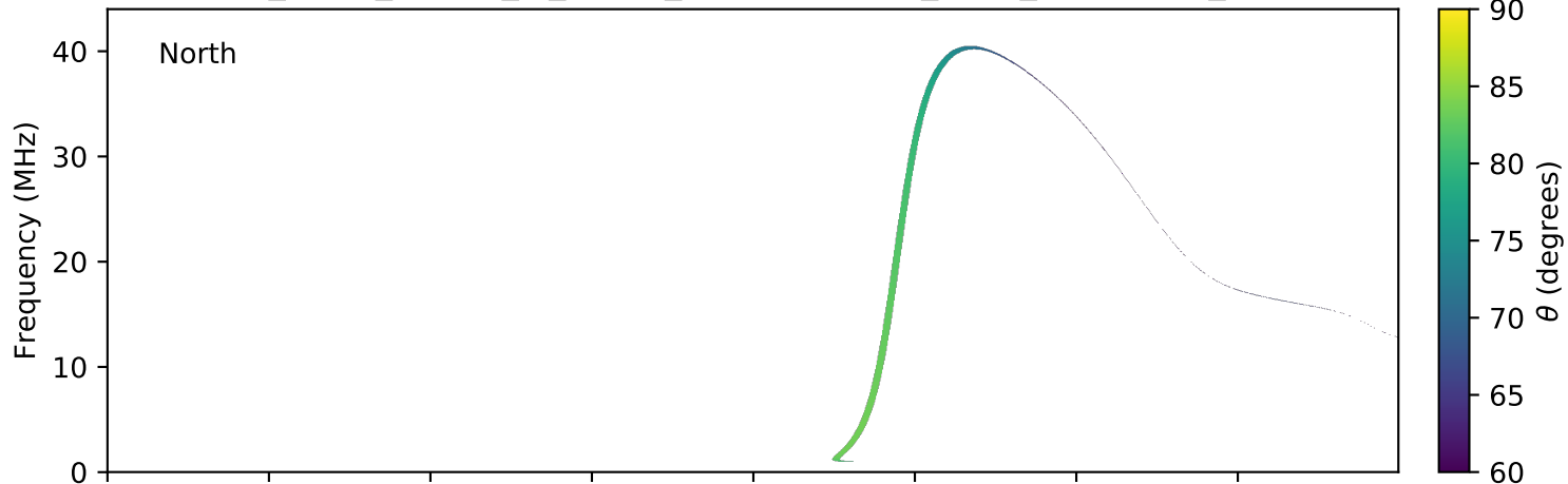
expres_earth_jupiter_io_jrm09_lossc-wid1deg_3kev_20070912_v01.cdf
