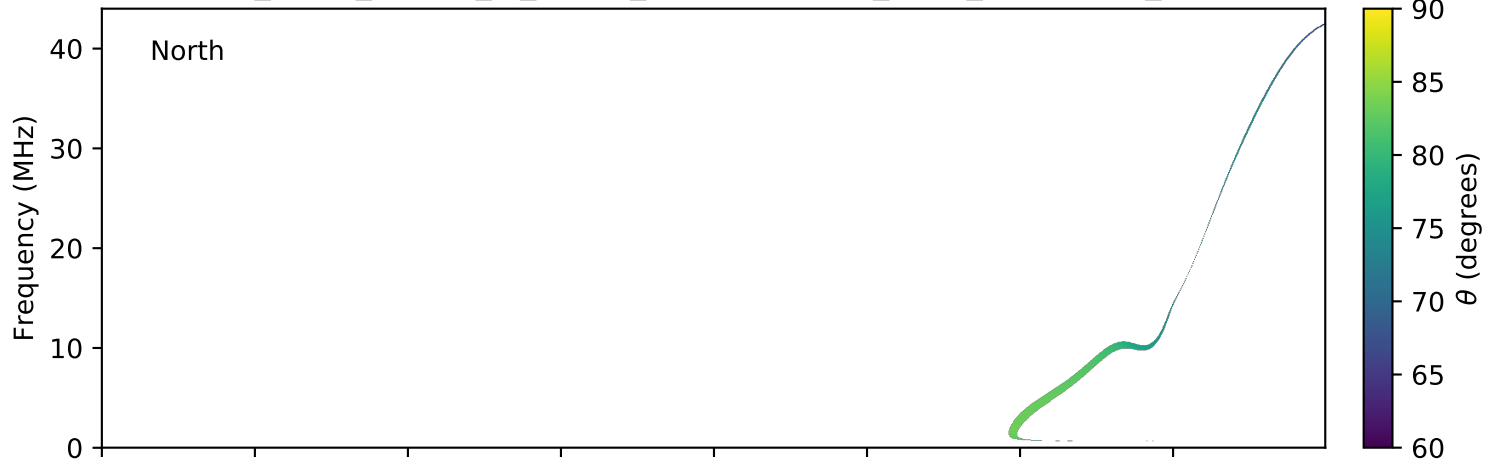
expres_earth_jupiter_io_jrm09_lossc-wid1deg_3kev_20070910_v01.cdf
