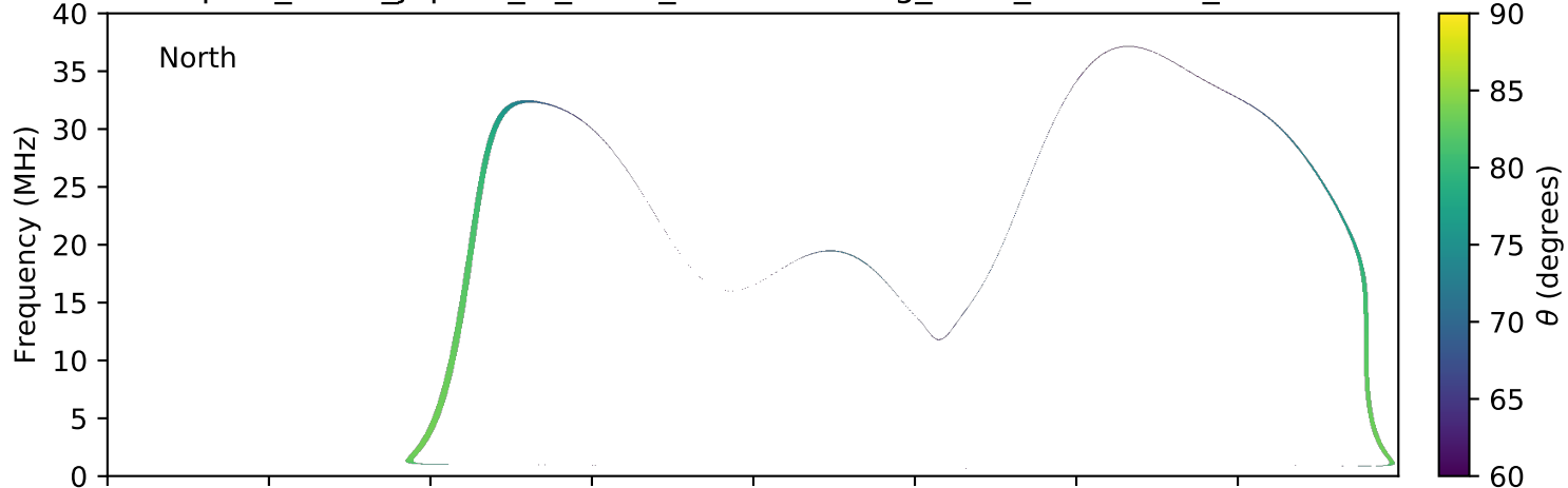
expres_earth_jupiter_io_isaac_lossc-wid1deg_3kev_20070930_v01.cdf
