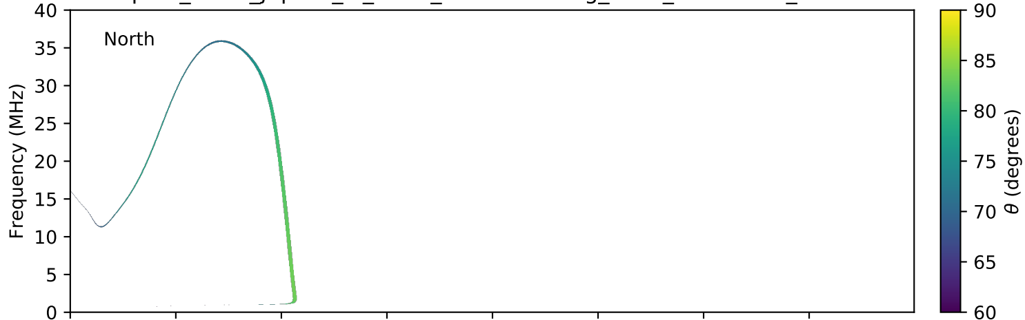
expres_earth_jupiter_io_isaac_lossc-wid1deg_3kev_20070929_v01.cdf
