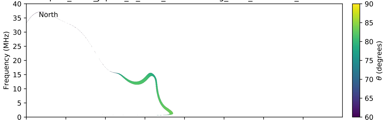
expres_earth_jupiter_io_isaac_lossc-wid1deg_3kev_20070927_v01.cdf
