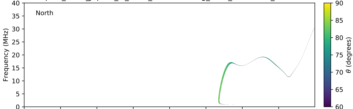
expres_earth_jupiter_io_isaac_lossc-wid1deg_3kev_20070926_v01.cdf
