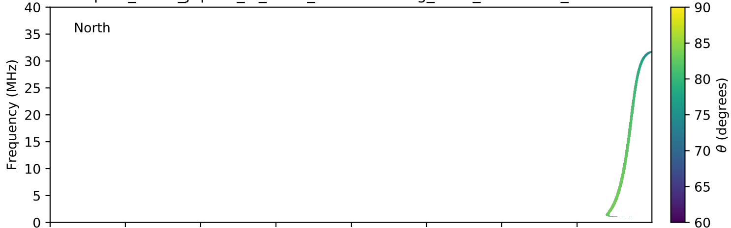
expres_earth_jupiter_io_isaac_lossc-wid1deg_3kev_20070924_v01.cdf
