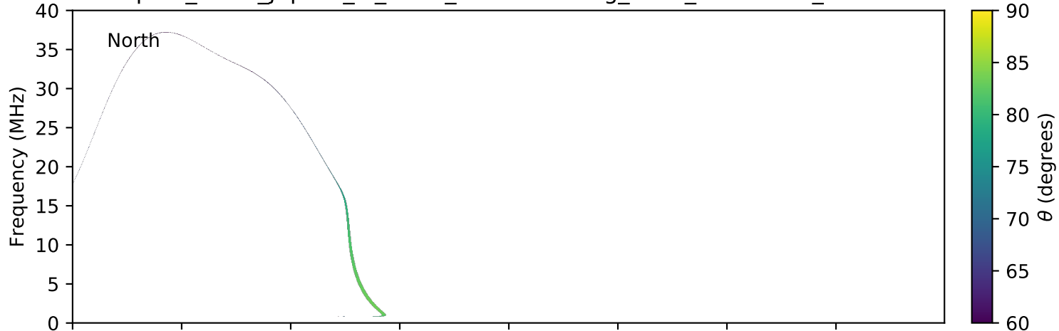
expres_earth_jupiter_io_isaac_lossc-wid1deg_3kev_20070920_v01.cdf
