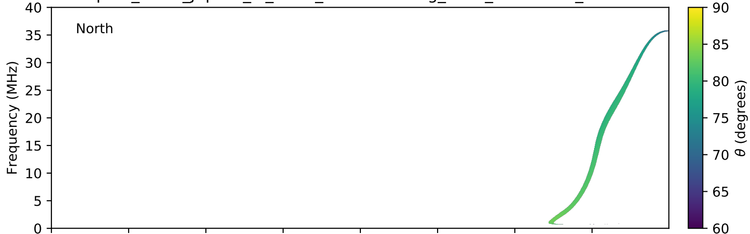
expres_earth_jupiter_io_isaac_lossc-wid1deg_3kev_20070917_v01.cdf
