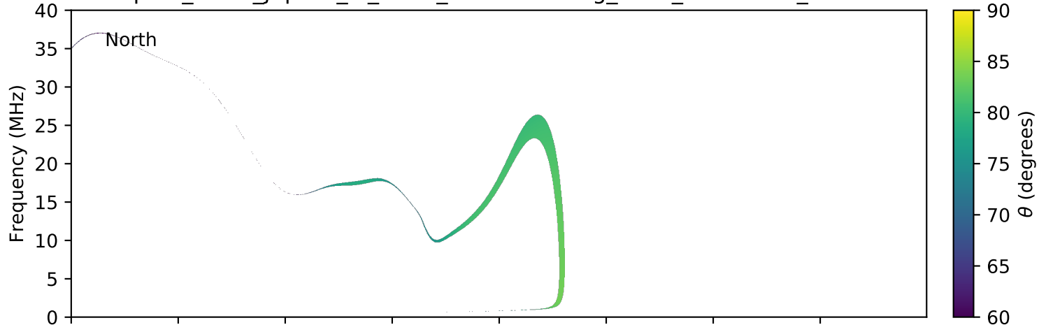
expres_earth_jupiter_io_isaac_lossc-wid1deg_3kev_20070911_v01.cdf
