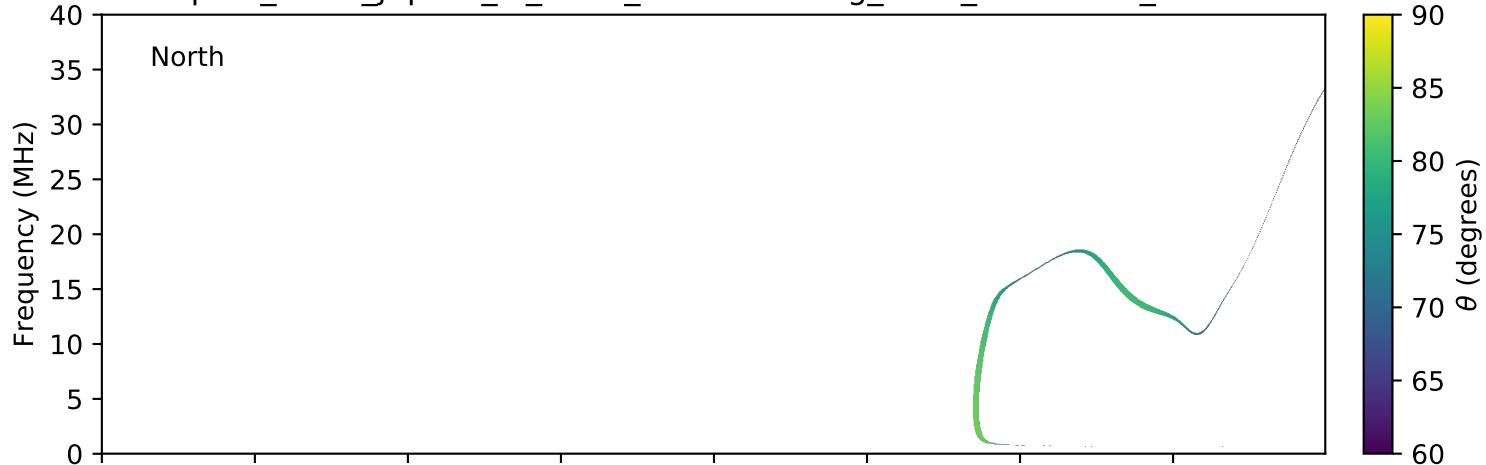
expres_earth_jupiter_io_isaac_lossc-wid1deg_3kev_20070910_v01.cdf
