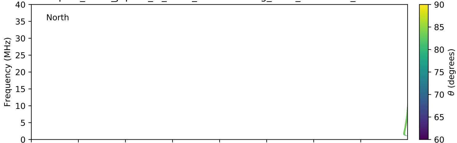
expres_earth_jupiter_io_isaac_lossc-wid1deg_3kev_20070908_v01.cdf
