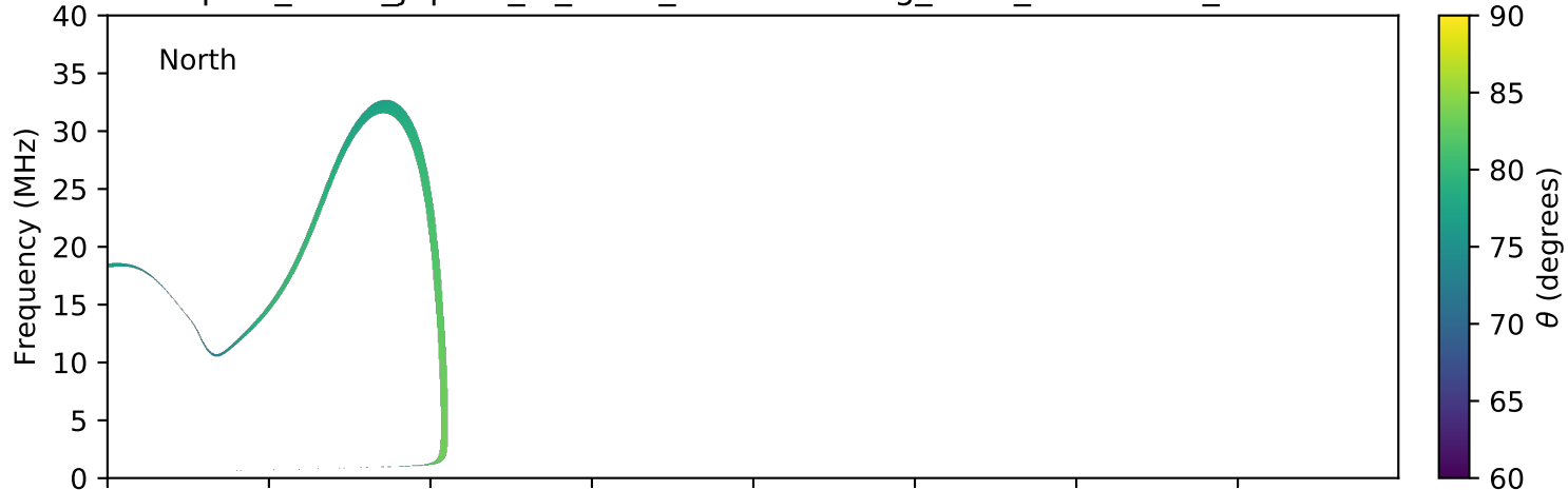
expres_earth_jupiter_io_isaac_lossc-wid1deg_3kev_20070906_v01.cdf
