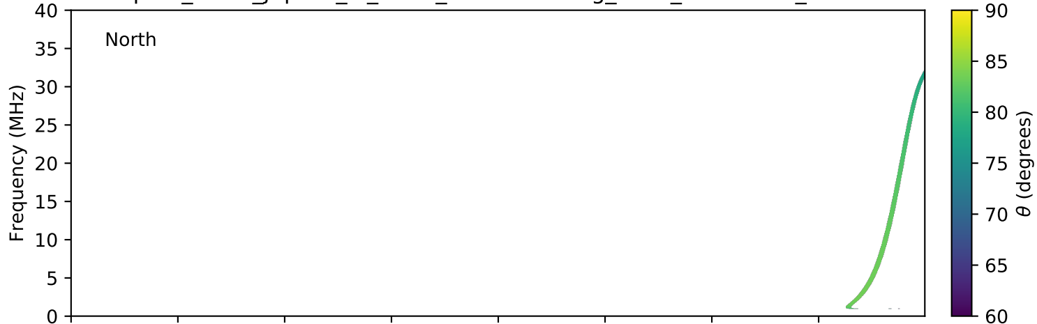
expres_earth_jupiter_io_isaac_lossc-wid1deg_3kev_20070901_v01.cdf
