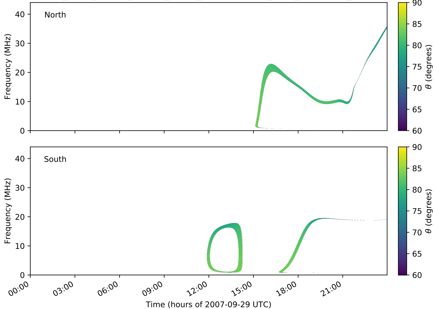
expres_earth_jupiter_europa_jrm09_lossc-wid1deg_3kev_20070929_v01.cdf
