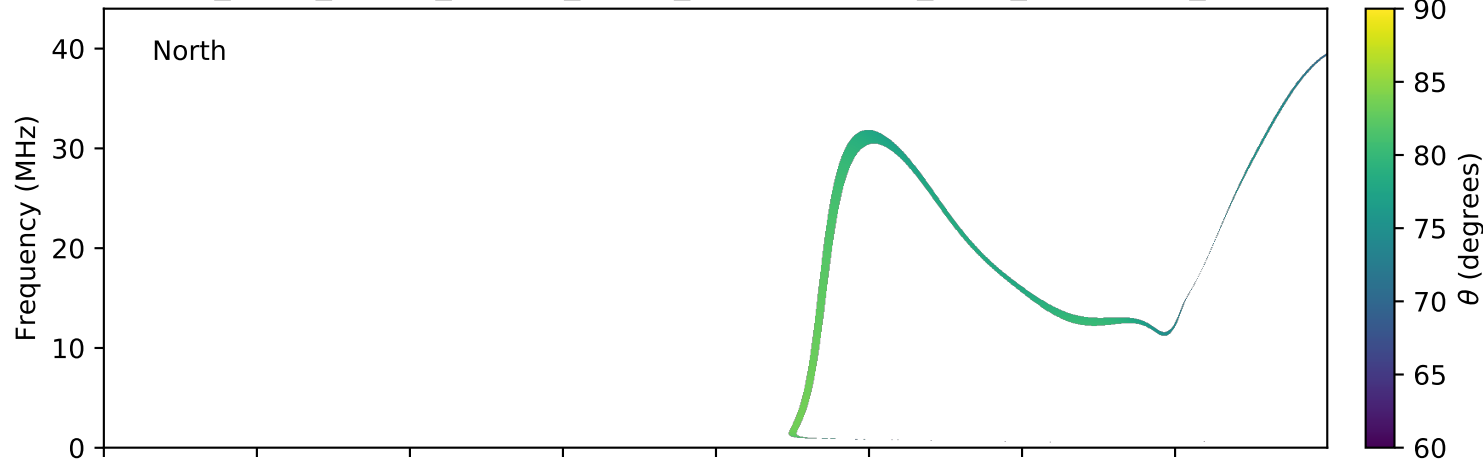
expres_earth_jupiter_europa_jrm09_lossc-wid1deg_3kev_20070922_v01.cdf
