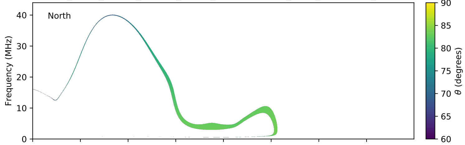
expres_earth_jupiter_europa_jrm09_lossc-wid1deg_3kev_20070920_v01.cdf
