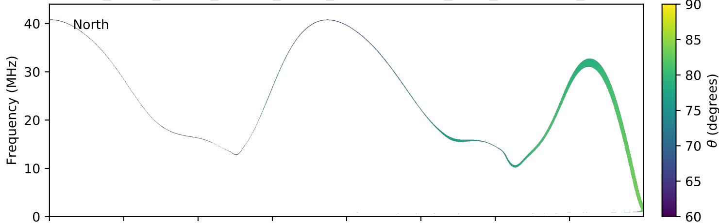
expres_earth_jupiter_europa_jrm09_lossc-wid1deg_3kev_20070916_v01.cdf
