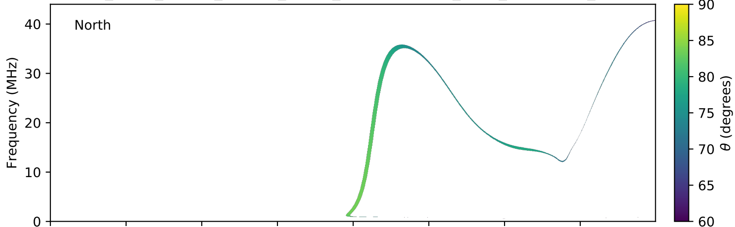
expres_earth_jupiter_europa_jrm09_lossc-wid1deg_3kev_20070915_v01.cdf
