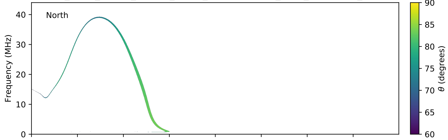
expres_earth_jupiter_europa_jrm09_lossc-wid1deg_3kev_20070913_v01.cdf
