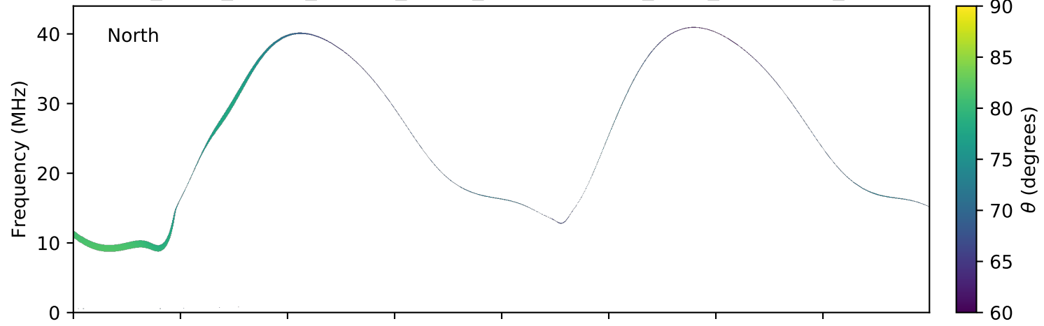
expres_earth_jupiter_europa_jrm09_lossc-wid1deg_3kev_20070912_v01.cdf
